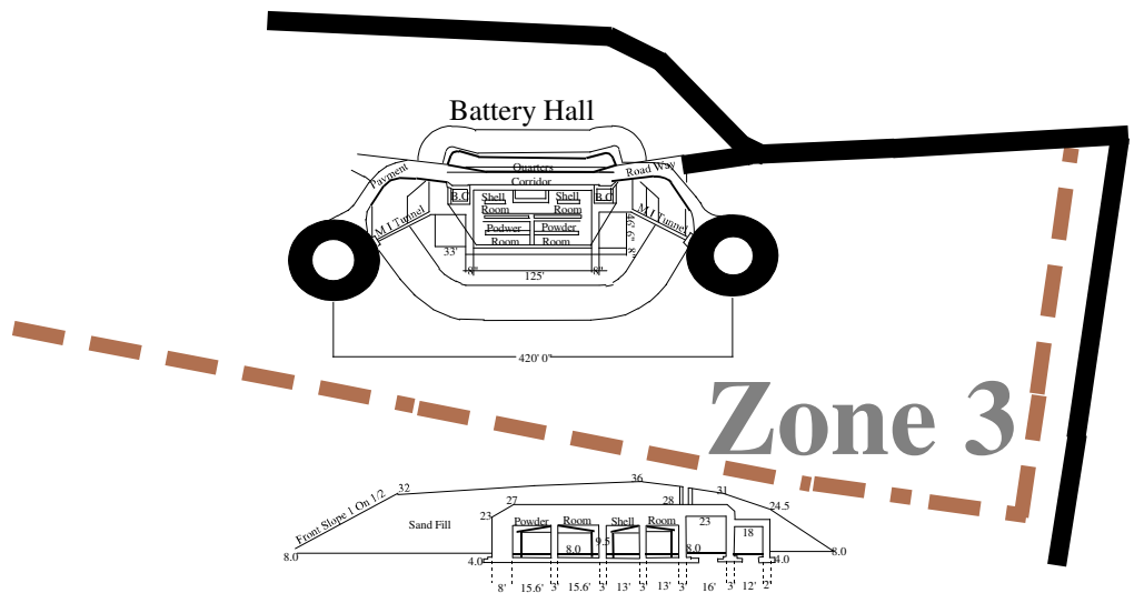
Cross Section Through Powder Magazin Of No 1 Gun Parallel To Capital Of Battery
