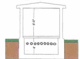
Section A-A Cable Hut
